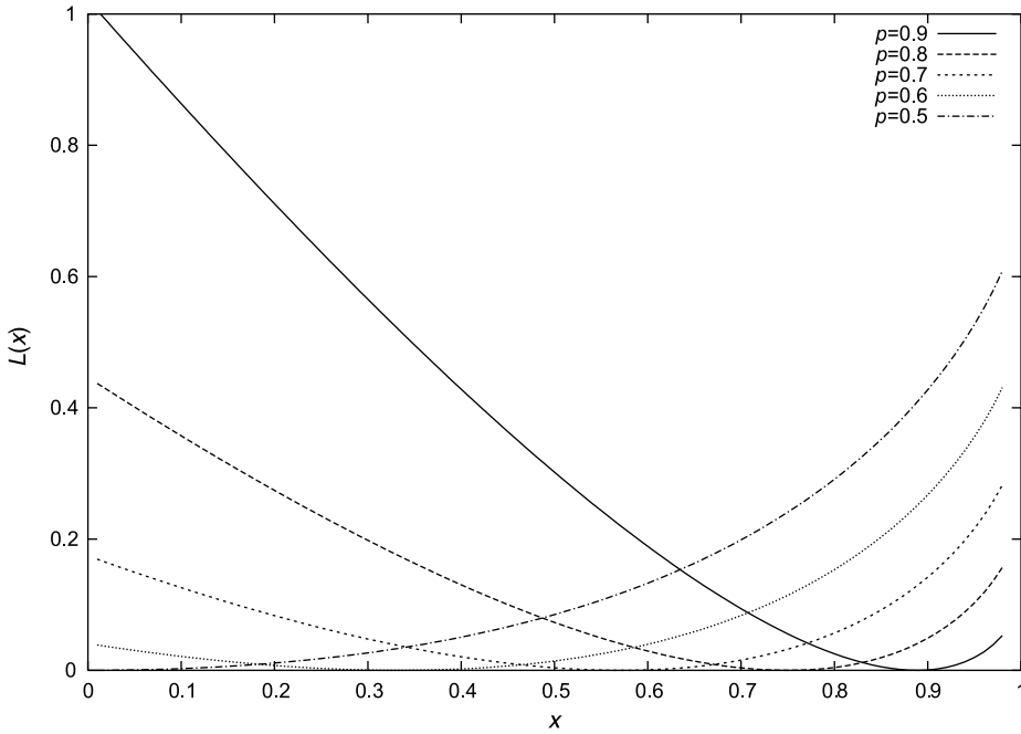
FIG. 3—Bernoulli-chooser rate-function p > 1/2 .
