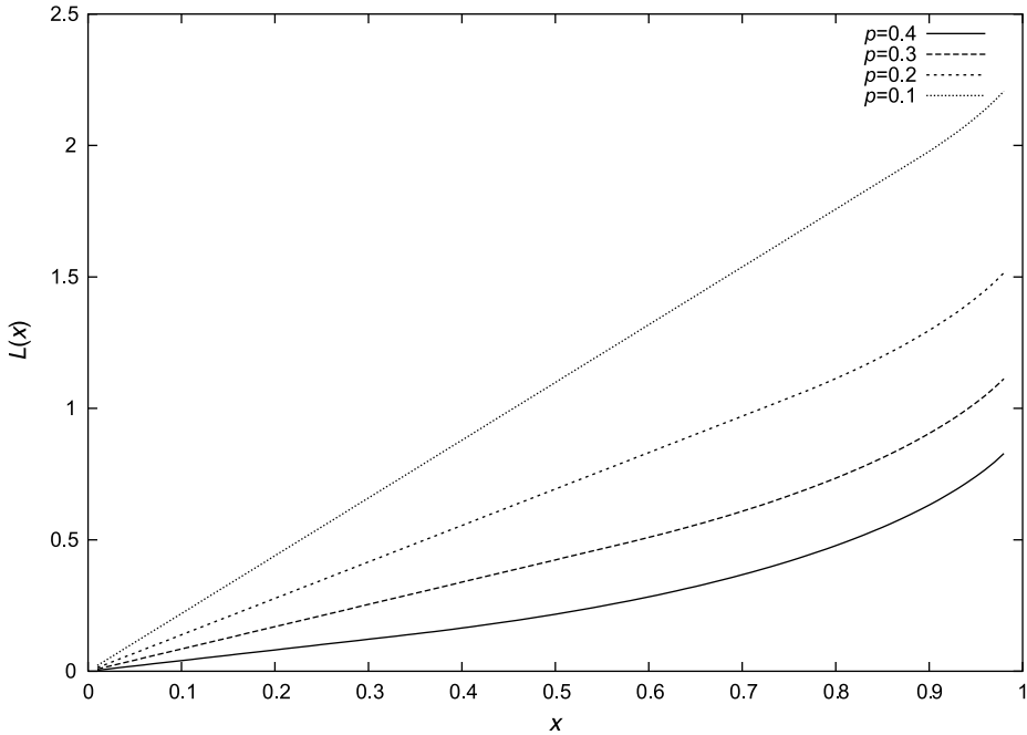
FIG. 2—Bernoulli-chooser rate-function, p \leq 1/2 .
