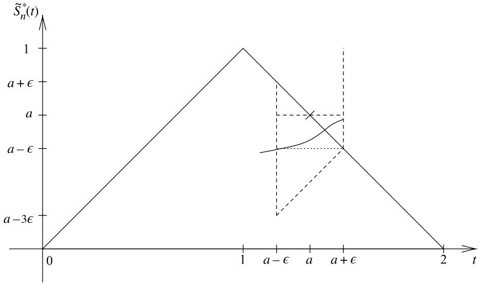
FIG. 1—Equivalence of events.
