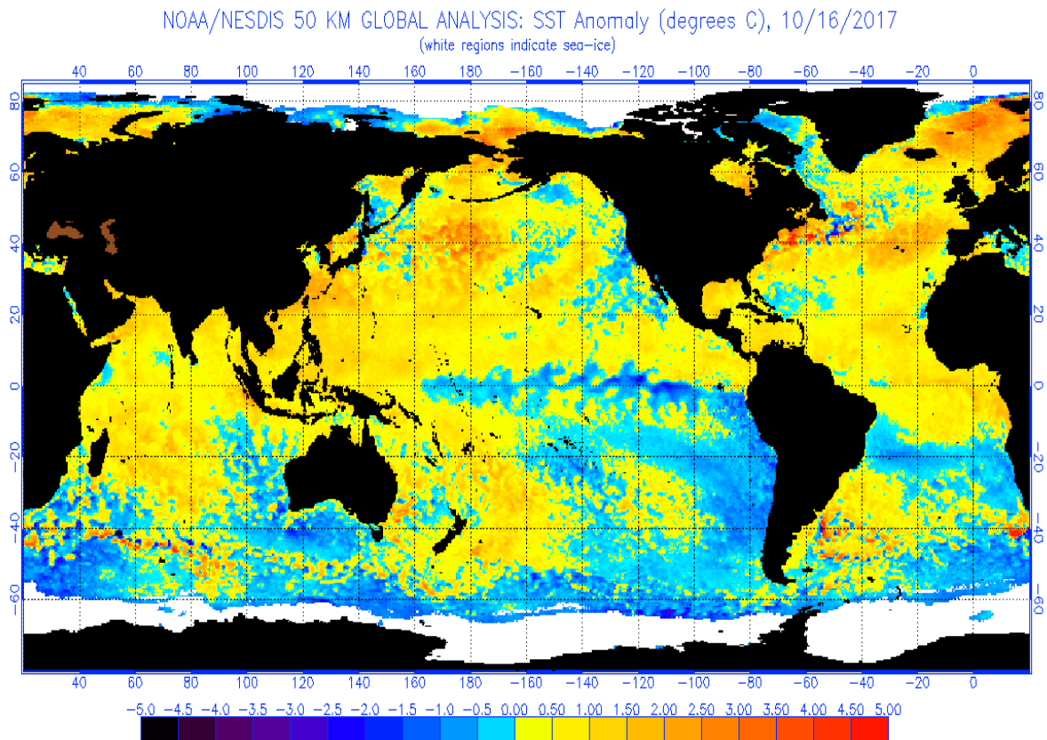
Figure 2. Global SST anomalies on 16 October 2017. Note the warm pool in the neighbourhood of the Azores with SST anomalies of +2°C. Source: http://www.ospo.noaa.gov/Products/ocean/sst/anomaly/
