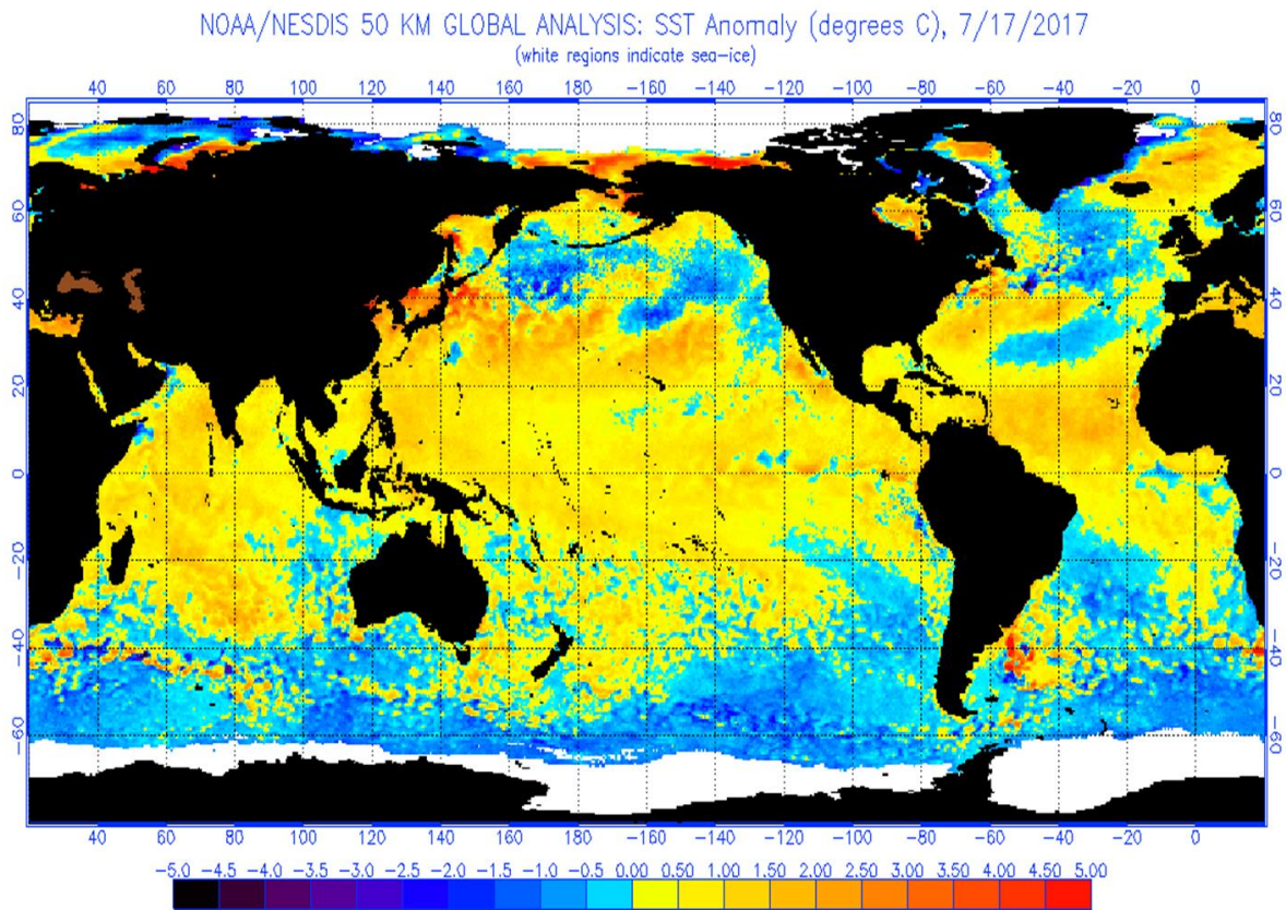
Figure 3. Global SST anomalies on 17 July 2017. Note the cold pool in the Azores/Ireland area with SST anomalies of -2°C. Source:
