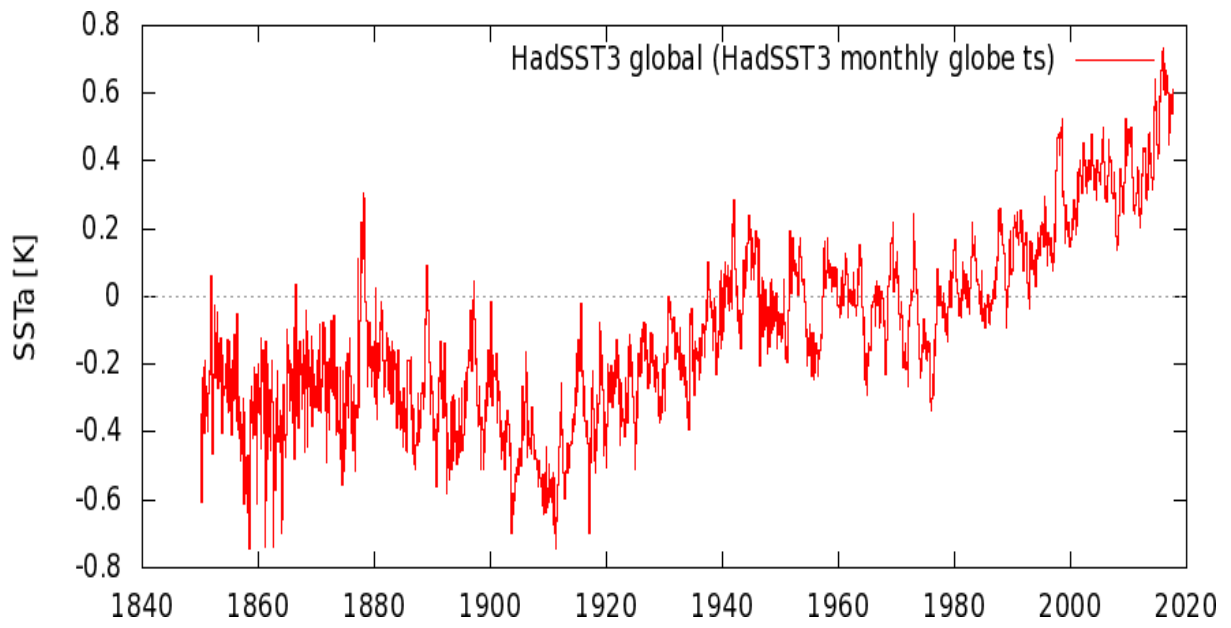
Figure 4. Monthly mean global SSTs (HasSST3) from 1850 to the present.
